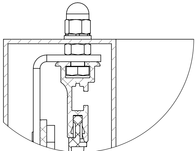
DETAIL E SCALE 1 : 1
