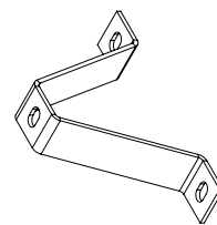
Omega H-55 bracket 29 x 54x 31 x 54 x 29 x 3 mm lg=20mm
