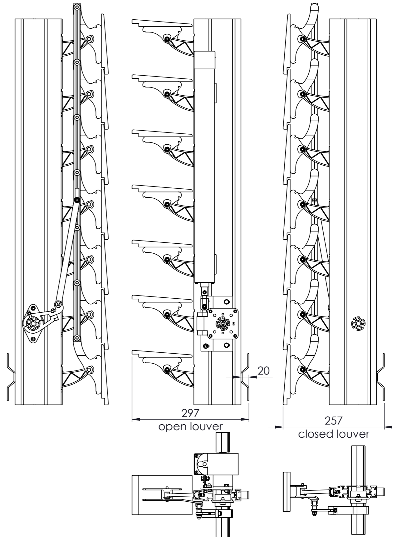
Rack arm 120mm
