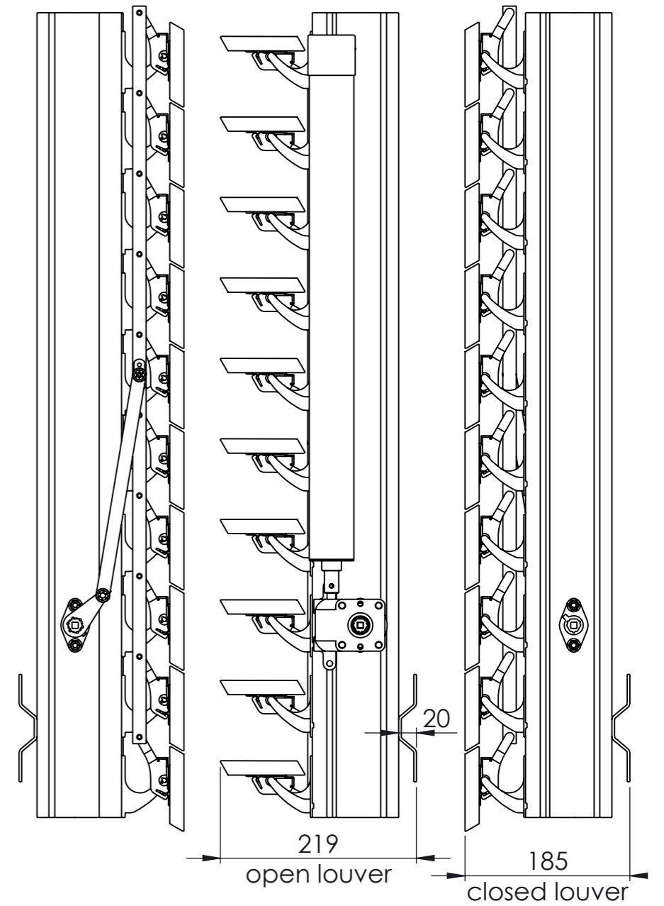
Rackarm 98 mm
