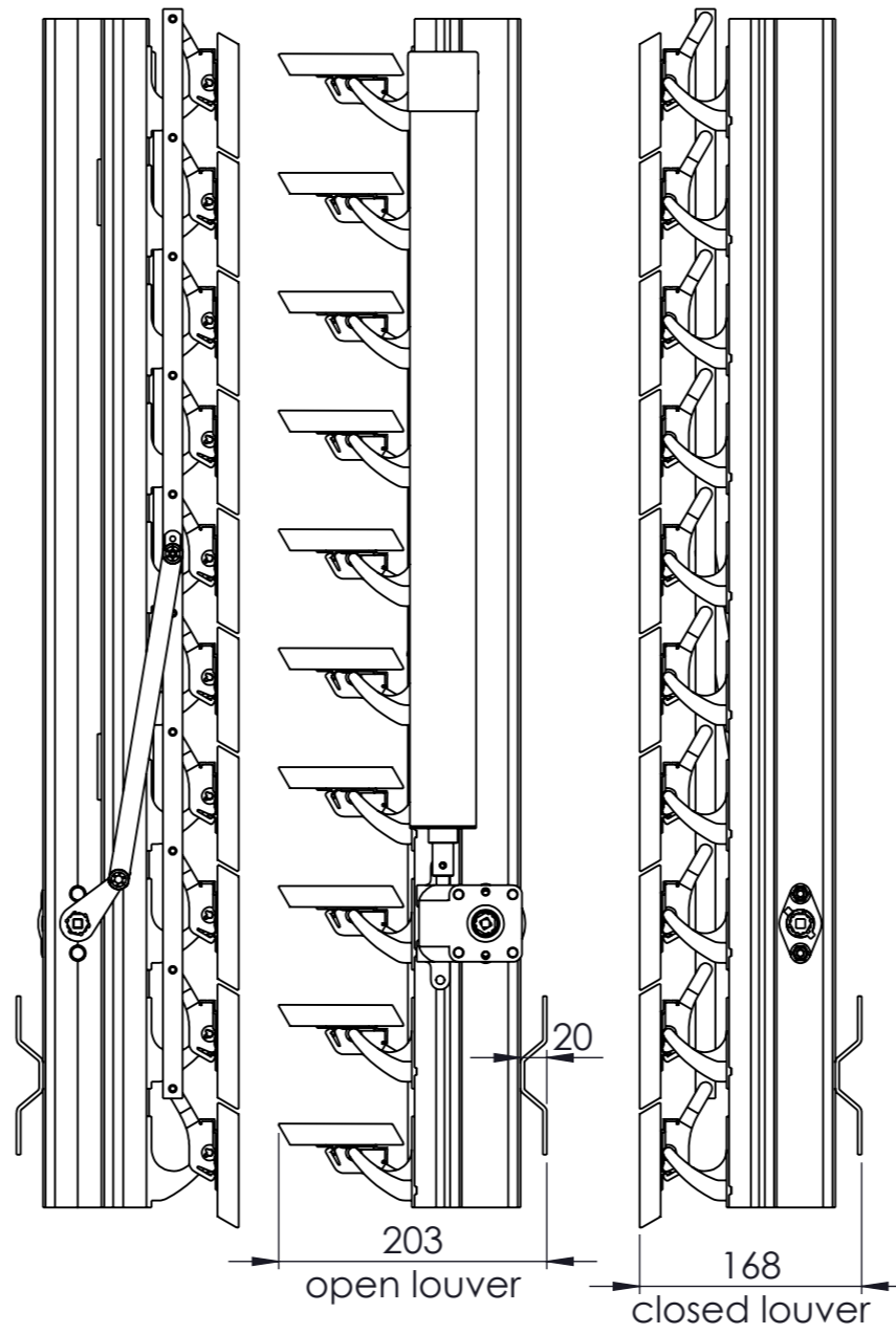
Rackarm 80 mm
