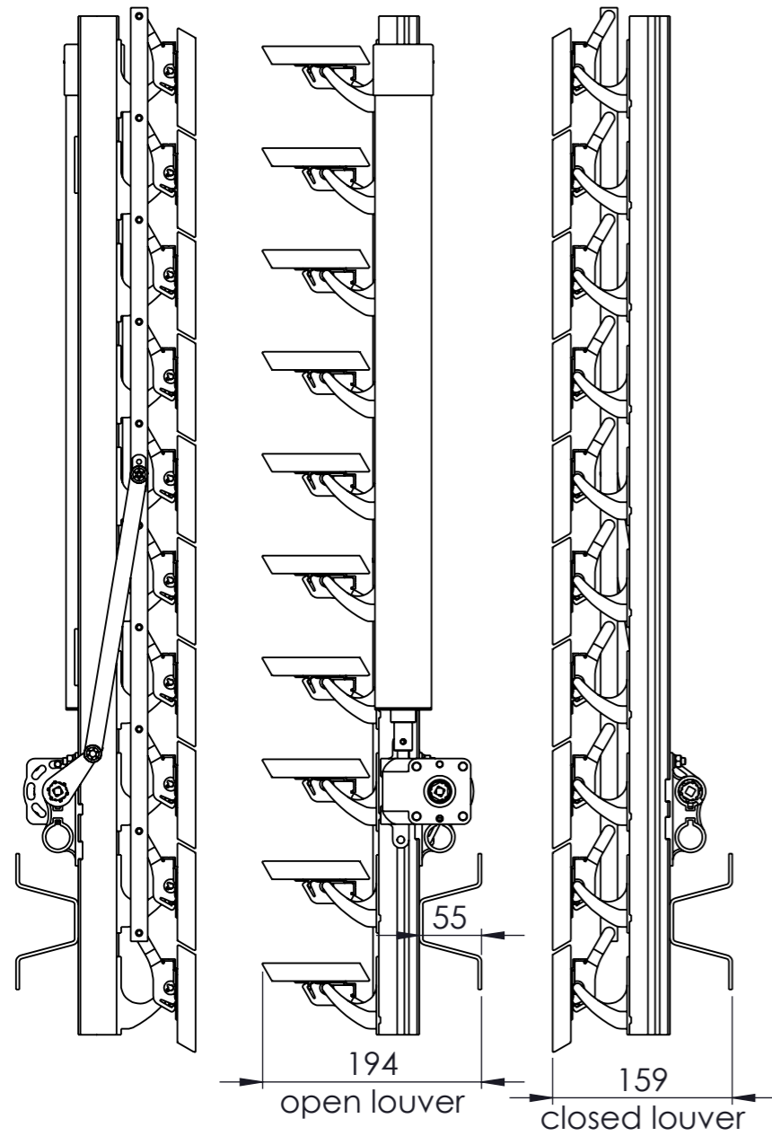
Rackarm 35 mm
