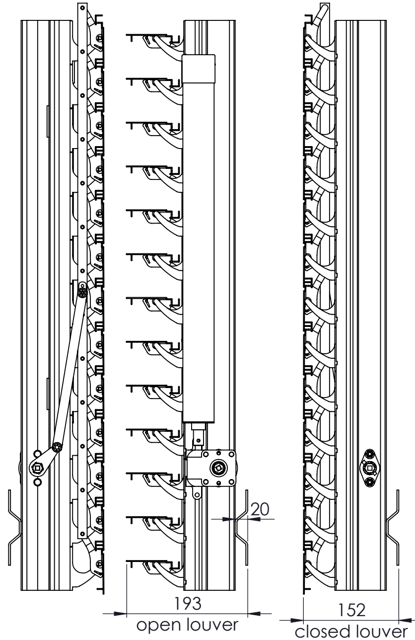
Rackarm 80 mm
