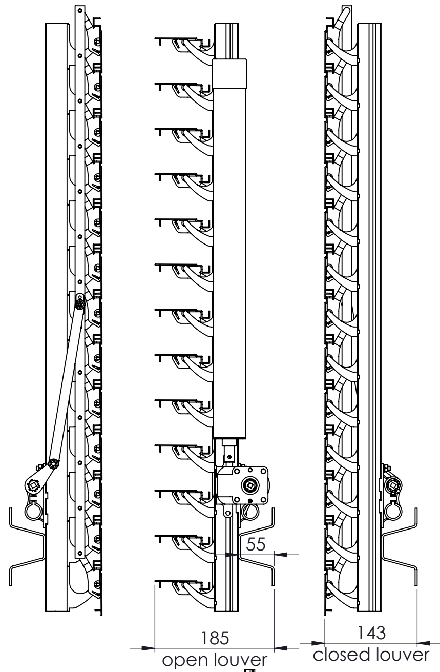
Rackarm 35 mm
