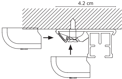
Smart Click Ceiling Bracket
