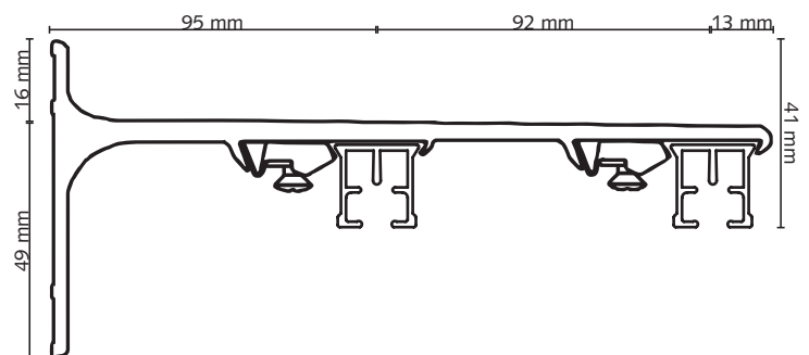
Aluminium Wall Bracket 20 cm Double
