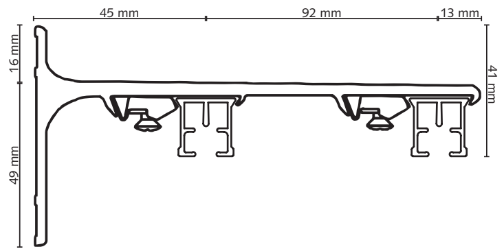
Aluminium Wall Bracket 20 cm Double
