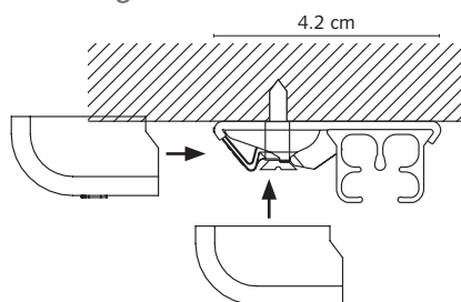
SK Ceiling Bracket
