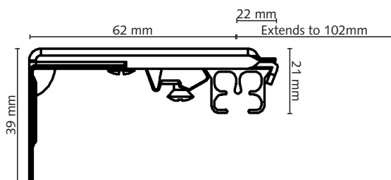
Double Adjustable Wall Bracket
