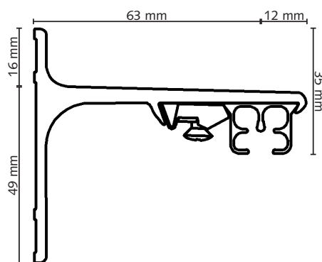
Aluminium Wall Bracket 10 cm
