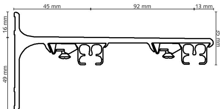
Aluminium Wall Bracket 15 cm Double
