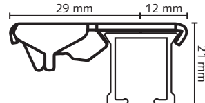
Smart Klick Ceiling Bracket
